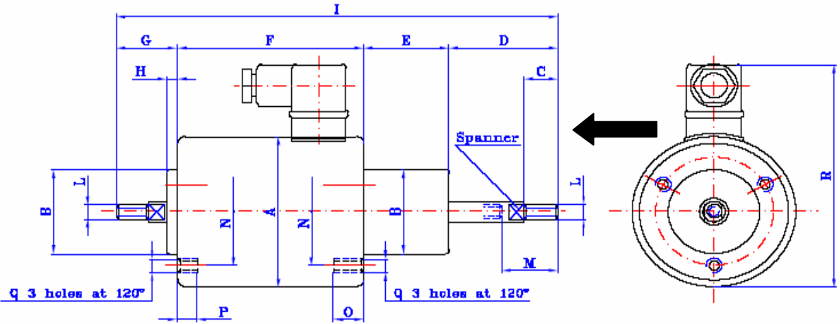
Dimensions (mm)
