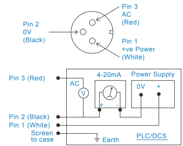
Connection Details
